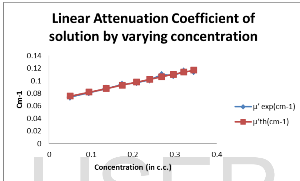
Fig. Linear Attenuation Coefficient of Oxalic Acid in Methanol solution by varying concentration for gamma energy 0.662 MeV.
